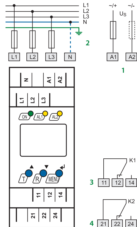
Figure 1 - VMD420 wiring diagram
